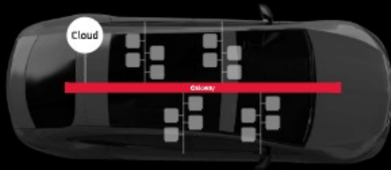
Typical Distributed Architecture
